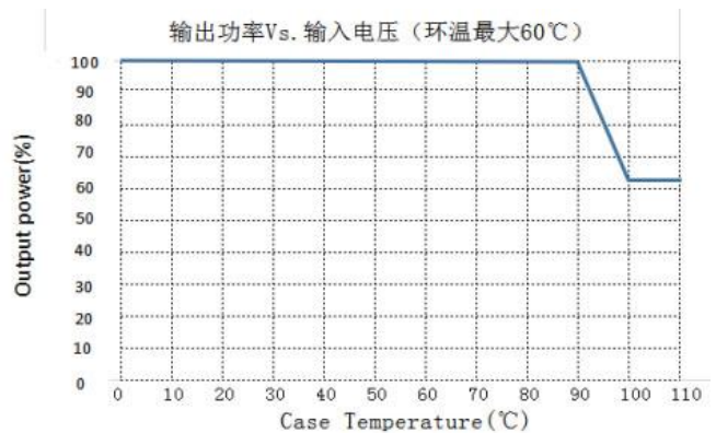
Output power VS Shell temperature
